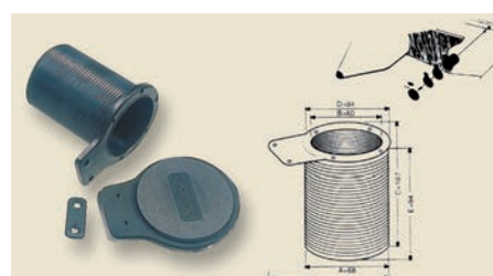
Cod. 327.05 Ø68 L.94 Autosvuotante per gommoni. Large drain socket for rubber boats.
