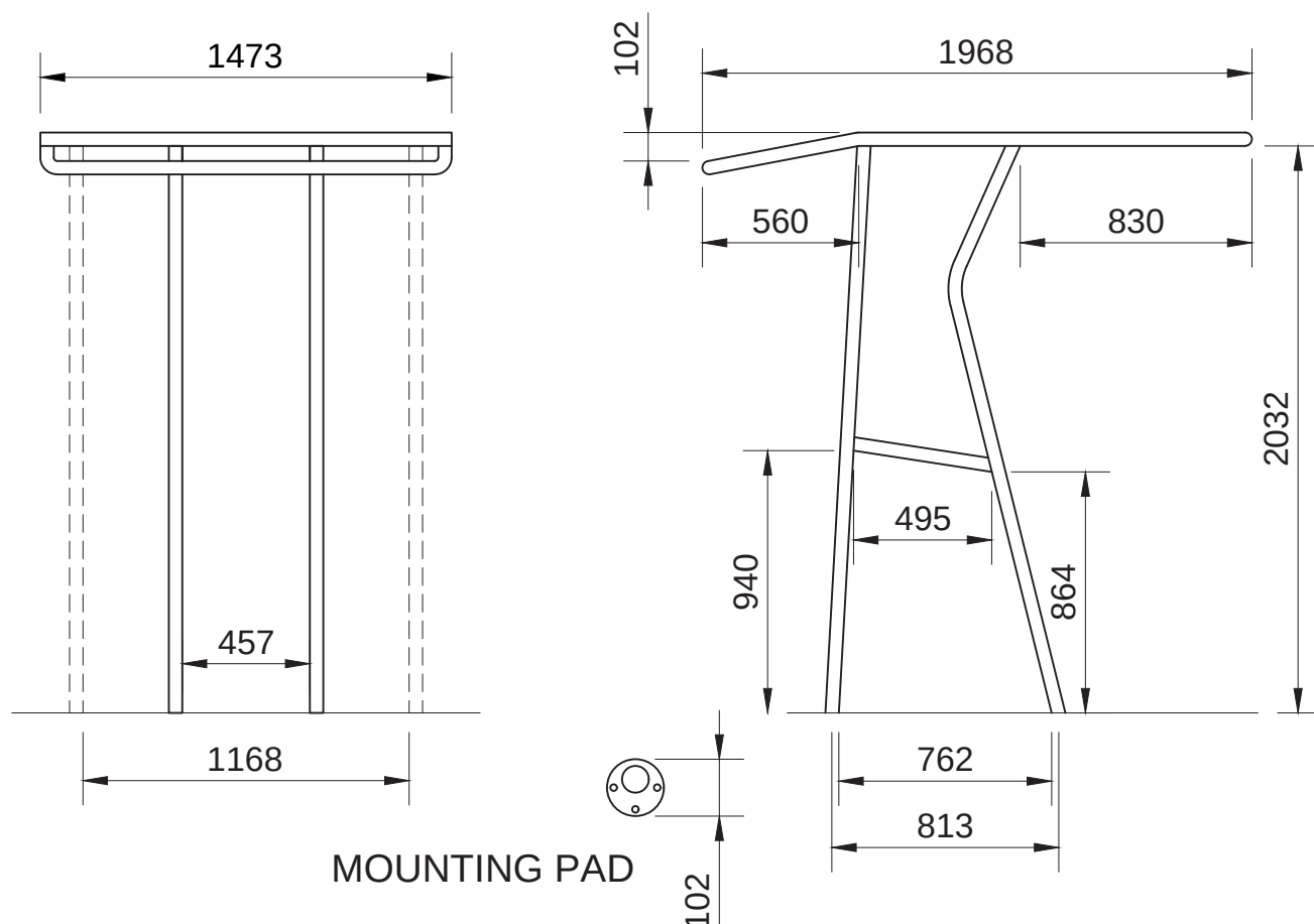
T-TOP ART.363.00 tubo Ø 48 mm / tube Ø 48 mm
