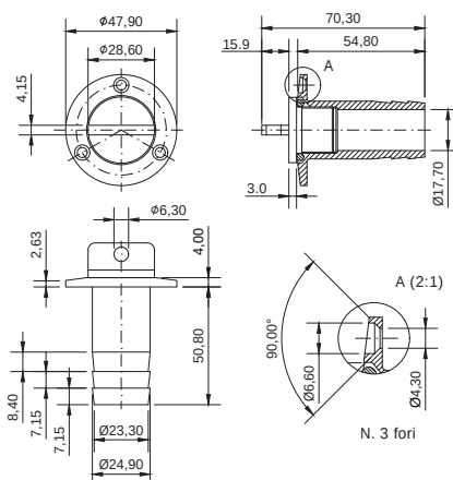
Scarichi a mare (ombrinali) in nylon. Thru-hull in nylon.
