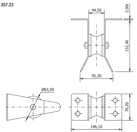
Musone inox Stainless steel platform bow roller Per ancore fino a 10 Kg For anchors up to 10 Kg
