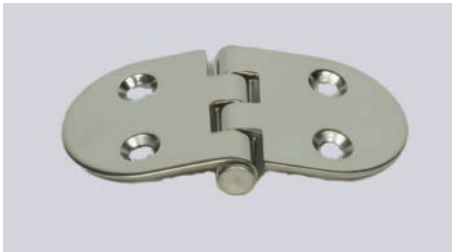
Cerniere in acc. inox lucidate; perno Ø 8 mm, spessore 2 mm. Polished stainless steel hinge; pivot Ø 8 mm, thickness 2 mm. Rovesciata Reversed pin
