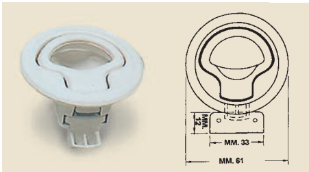
Cod. 343.10 Maniglia Ø 61. Cod. 343.10 Flat pull Ø 61.
